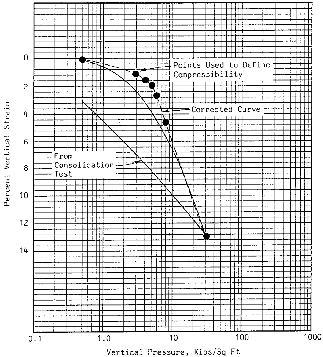
Figure 5.2 Soil Compressibility curve for Example Problem 1
