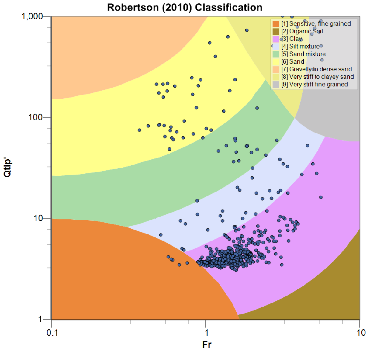
Figure 4 - Classification Chart
