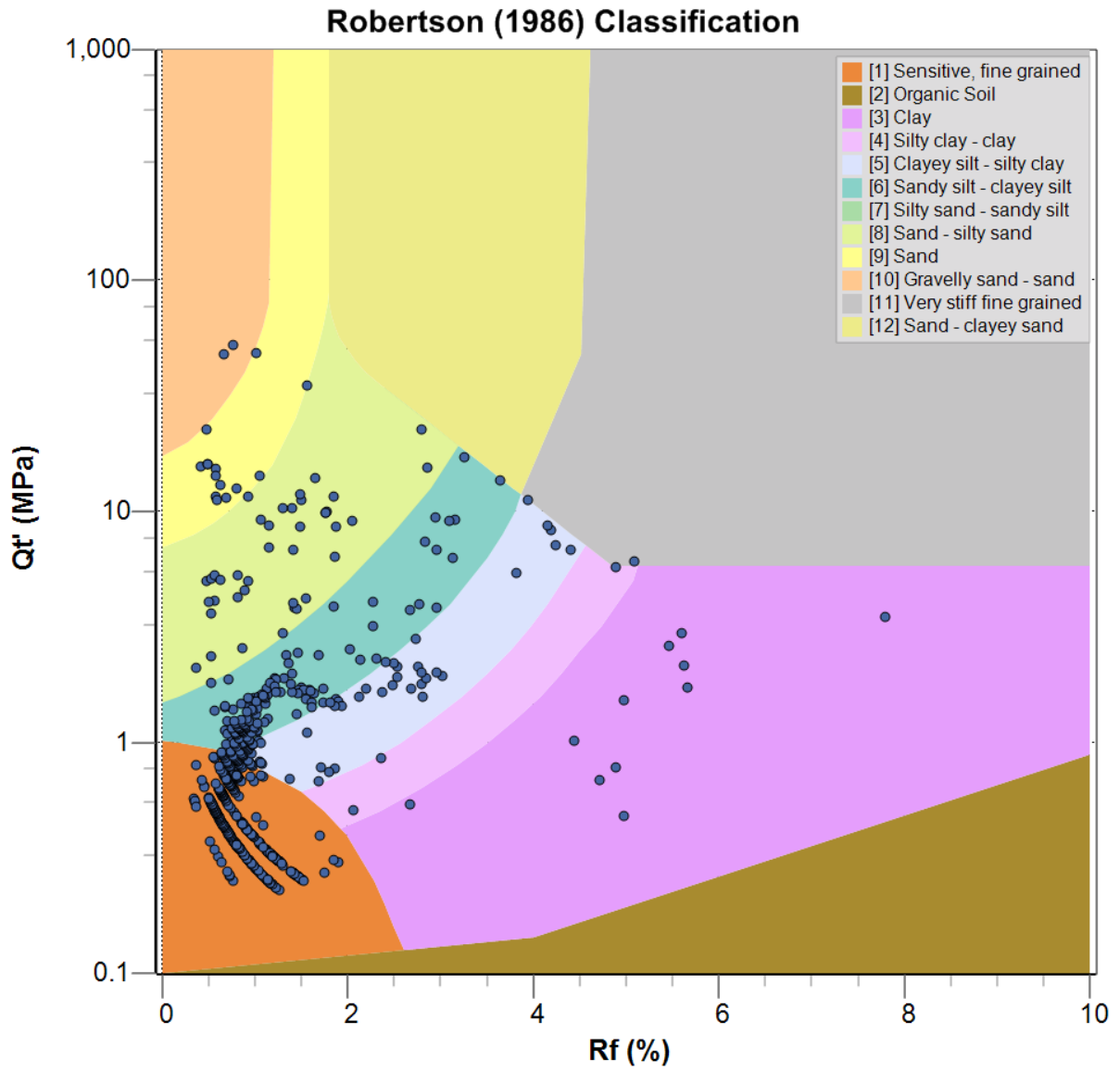
Figure 3 - Classification Chart
