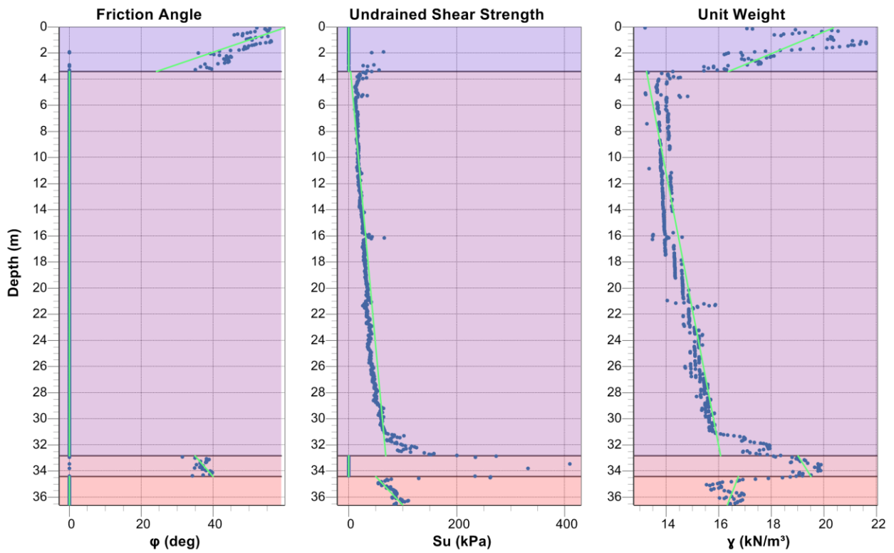
Figure 2 - Selected layering and soil properties
